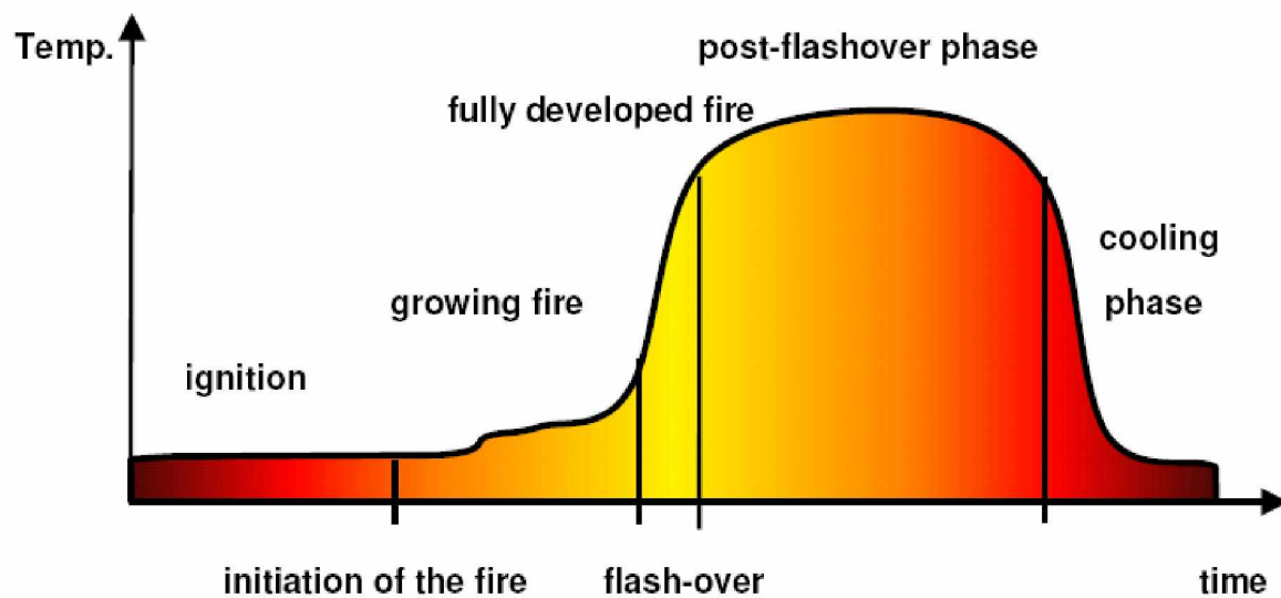
Fig. 1 : fire model (after Troitzsch [5], Beard [6] et.al.)
